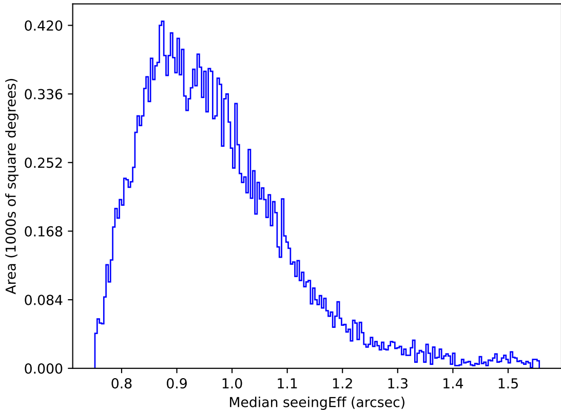
ddf_acor_sf10_lsf20_lsr20_v3.4_10yrs Yr 1 z band: Median seeingEff
