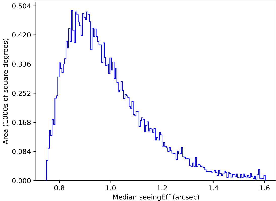
ddf_acor_sf10_lsf20_lsr20_v3.4_10yrs Yr 1 r band: Median seeingEff
