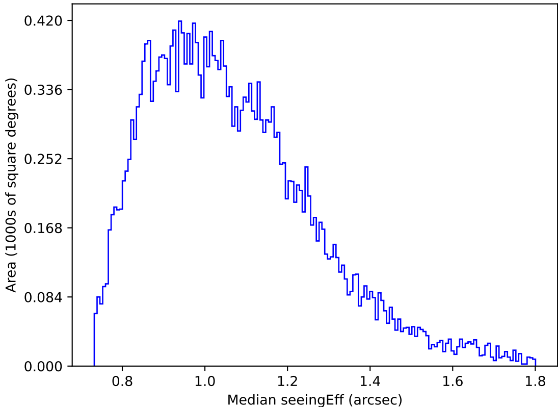
ddf_acor_sf10_lsf20_lsr20_v3.4_10yrs Yr 1 g band: Median seeingEff
