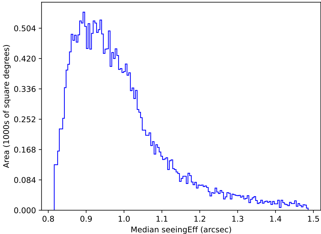
ddf_acor_sf10_lsf20_lsr20_v3.4_10yrs Yr 1 all bands: Median seeingEff
