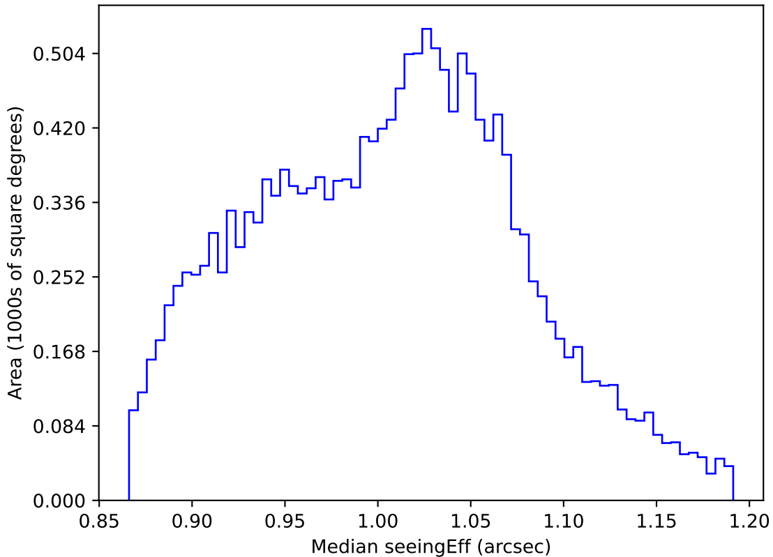
ddf_acor_sf10_lsf20_lsr20_v3.4_10yrs WFD z band: Median seeingEff
