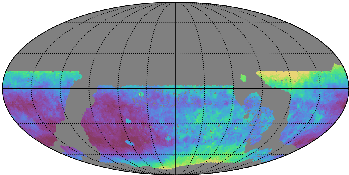
ddf_acor_sf10_lsf20_lsr20_v3.4_10yrs WFD i band: Median seeingEff
