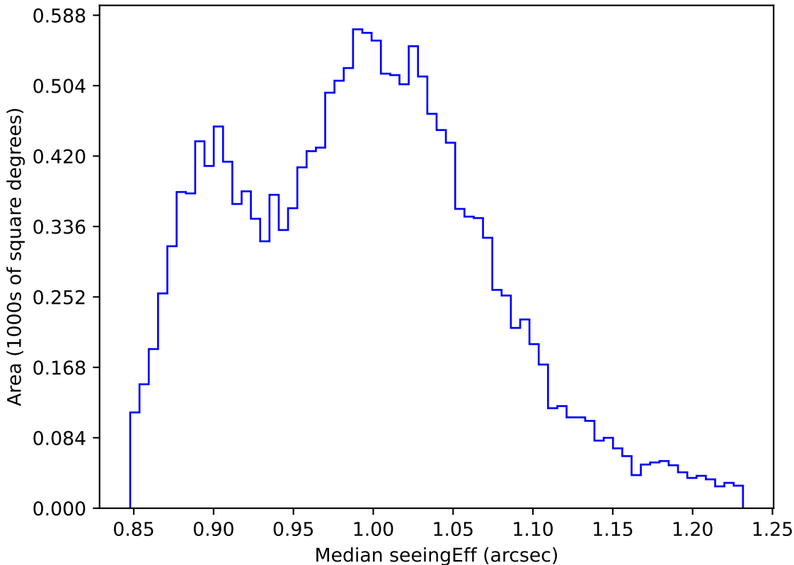
ddf_acor_sf10_lsf20_lsr20_v3.4_10yrs WFD i band: Median seeingEff
