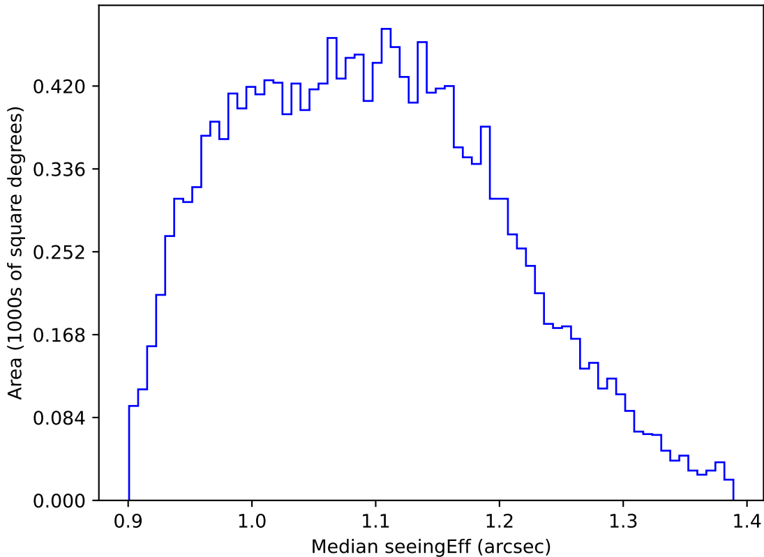
ddf_acor_sf10_lsf20_lsr20_v3.4_10yrs WFD g band: Median seeingEff
