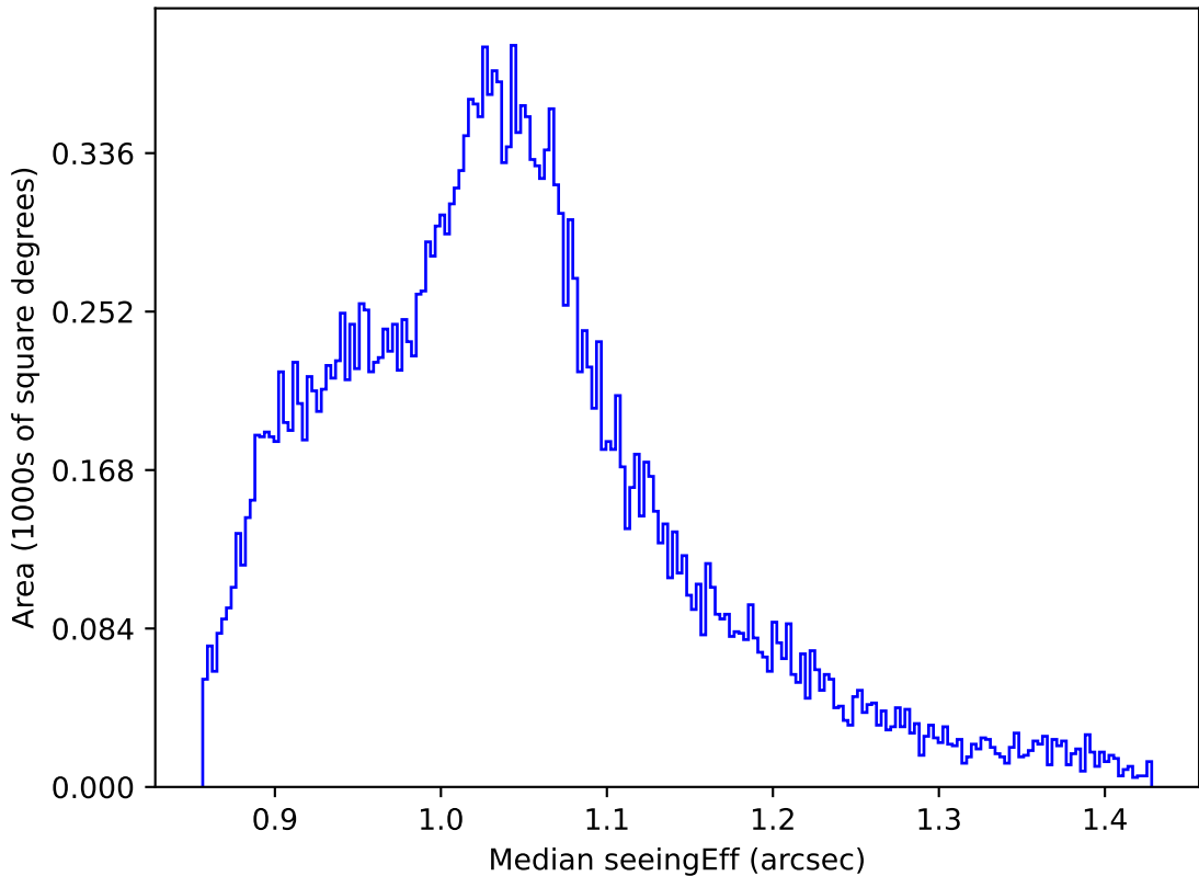
ddf_acor_sf10_lsf20_lsr20_v3.4_10yrs All sky z band: Median seeingEff
