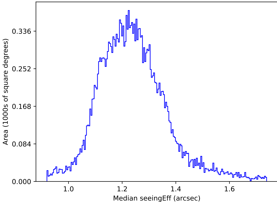
ddf_acor_sf10_lsf20_lsr20_v3.4_10yrs All sky u band: Median seeingEff
