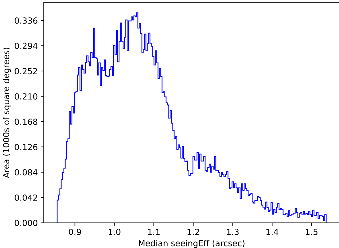
ddf_acor_sf10_lsf20_lsr20_v3.4_10yrs All sky r band: Median seeingEff
