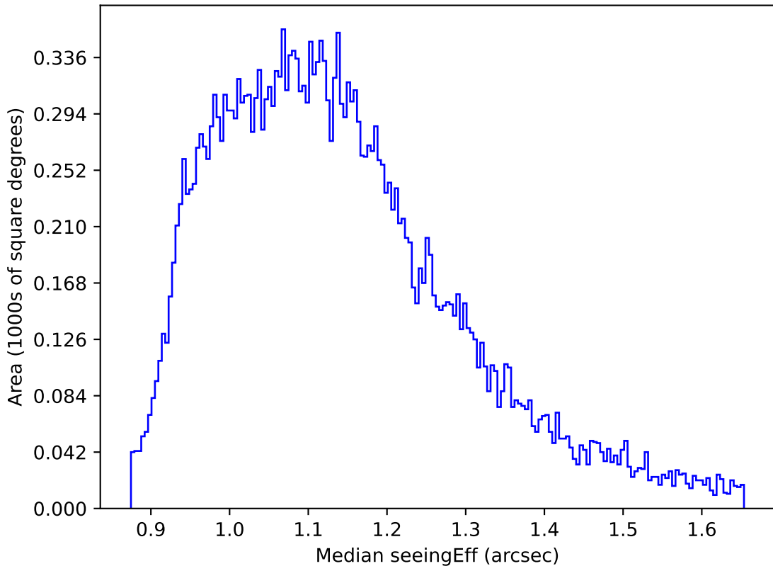
ddf_acor_sf10_lsf20_lsr20_v3.4_10yrs All sky g band: Median seeingEff
