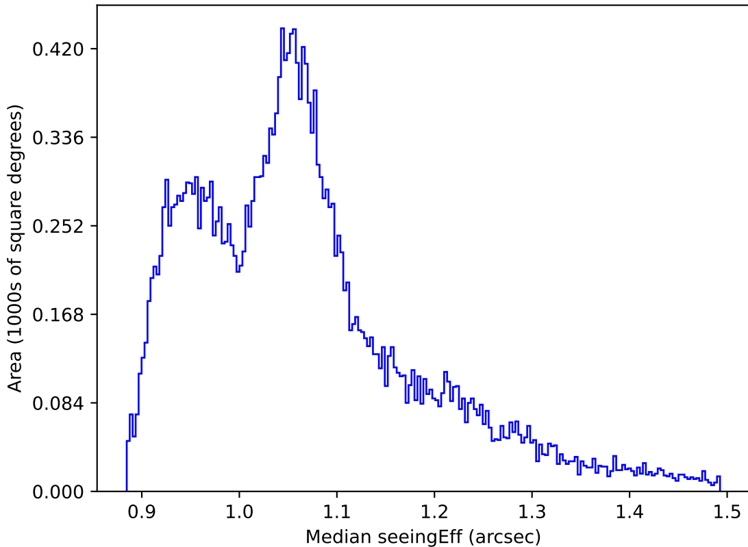
ddf_acor_sf10_lsf20_lsr20_v3.4_10yrs All sky all bands: Median seeingEff
