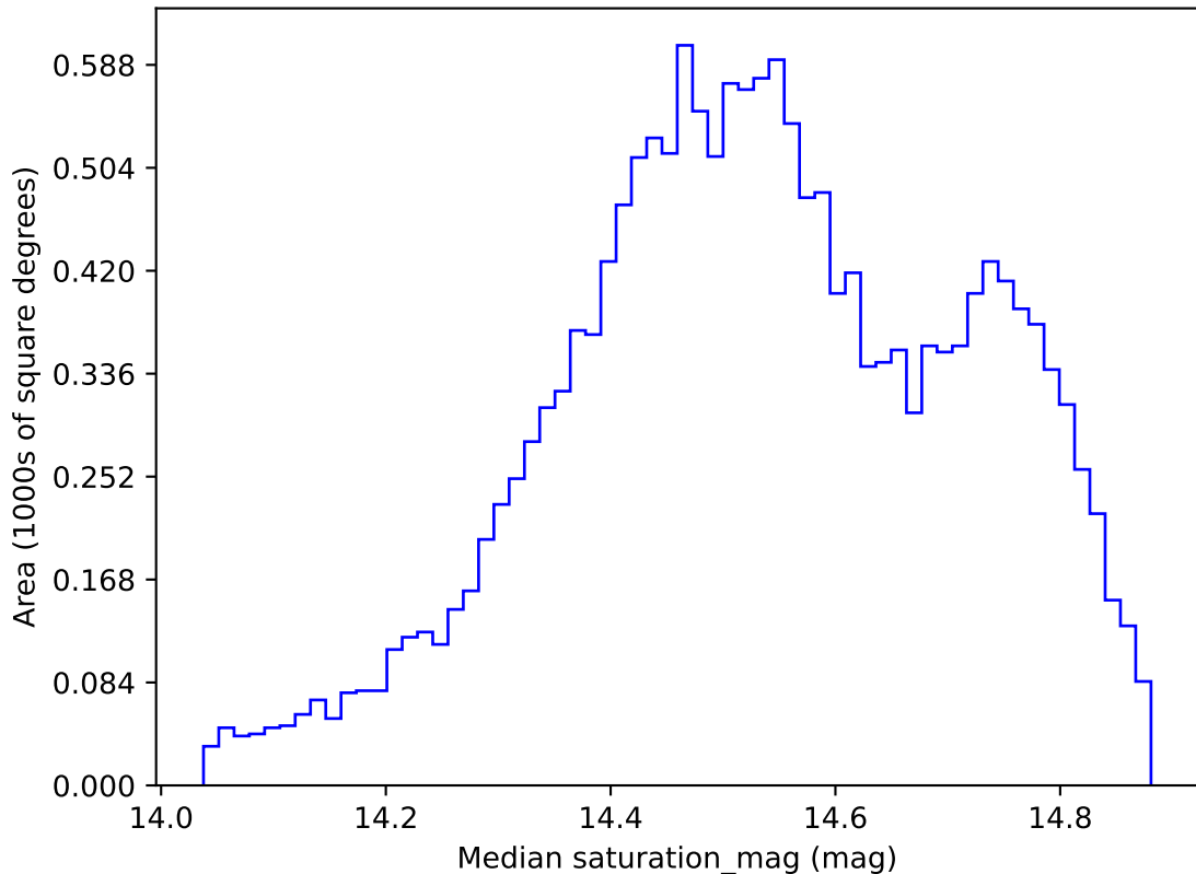
ddf_acor_sf10_lsf20_lsr20_v3.4_10yrs WFD i band: Median saturation_mag
