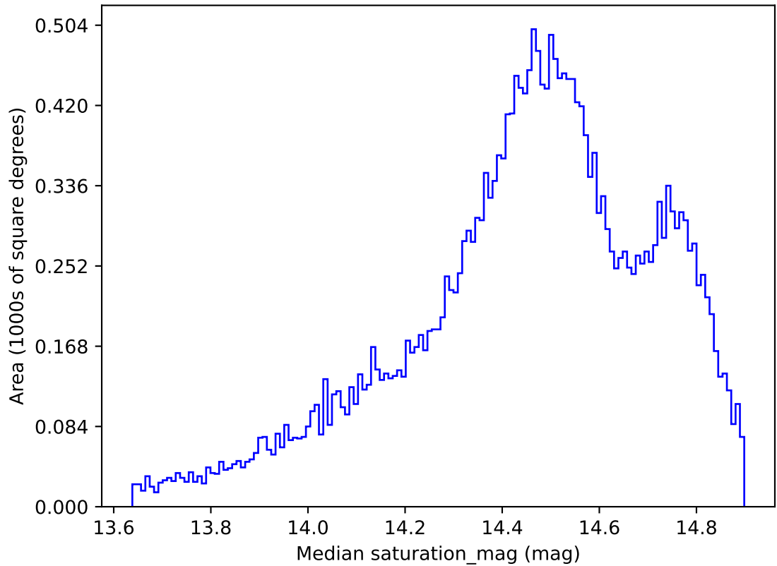
ddf_acor_sf10_lsf20_lsr20_v3.4_10yrs All sky i band: Median saturation_mag
