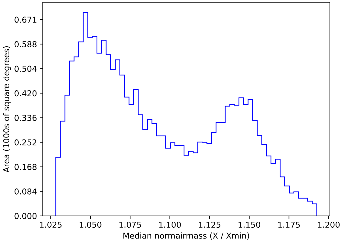
ddf_acor_sf10_lsf20_lsr20_v3.4_10yrs WFD y band: Median normairmass
