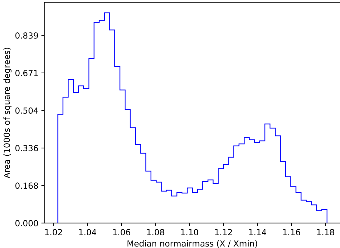
ddf_acor_sf10_lsf20_lsr20_v3.4_10yrs WFD all bands: Median normairmass
