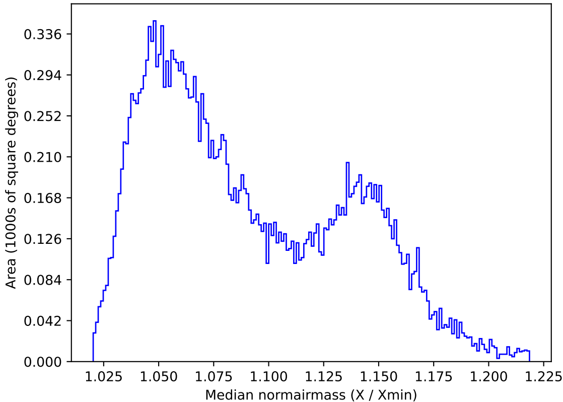
ddf_acor_sf10_lsf20_lsr20_v3.4_10yrs All sky y band: Median normairmass
