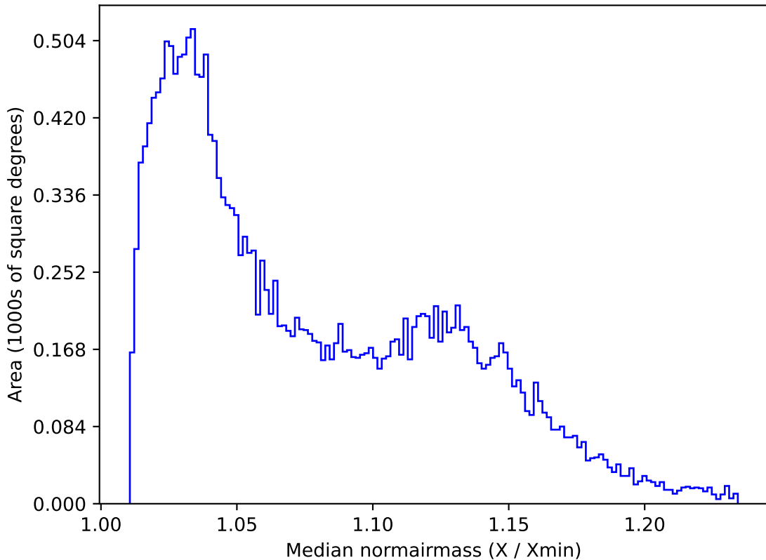
ddf_acor_sf10_lsf20_lsr20_v3.4_10yrs All sky u band: Median normairmass
