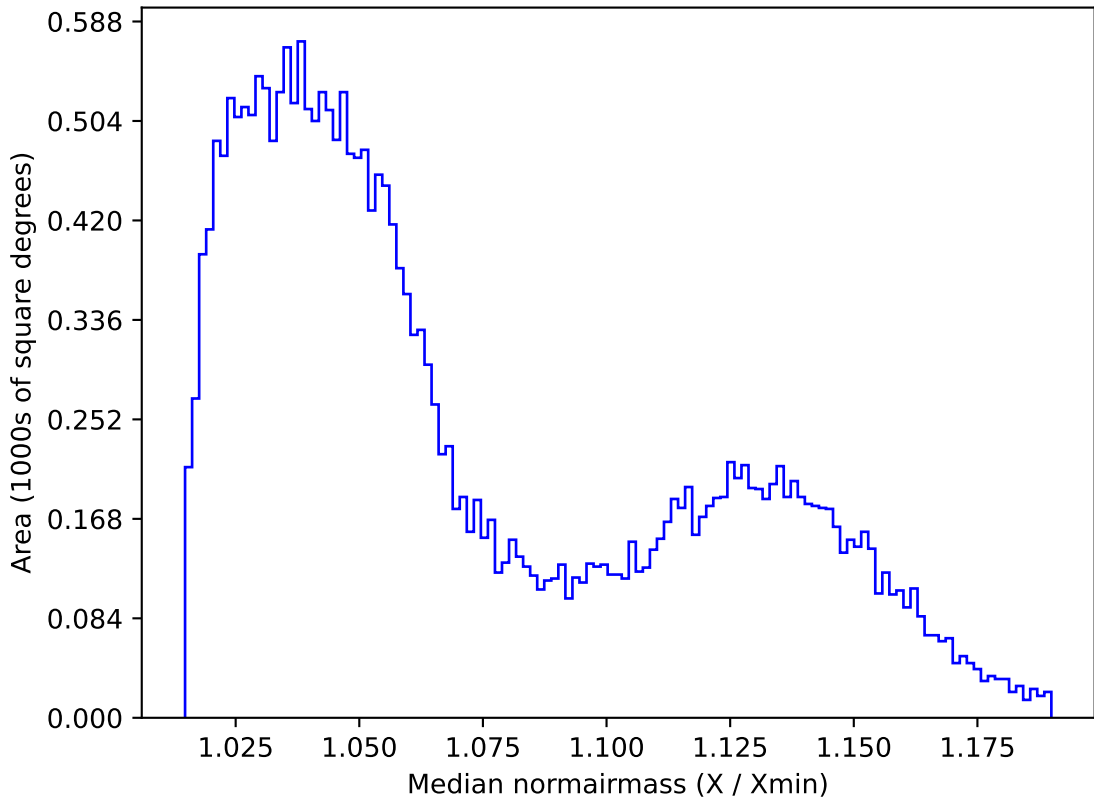
ddf_acor_sf10_lsf20_lsr20_v3.4_10yrs All sky r band: Median normairmass
