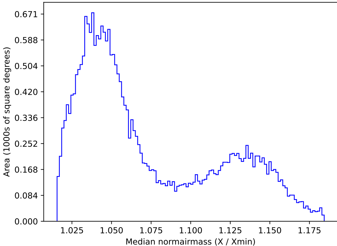
ddf_acor_sf10_lsf20_lsr20_v3.4_10yrs All sky i band: Median normairmass
