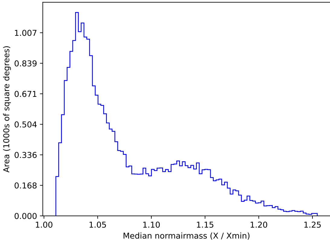
ddf_acor_sf10_lsf20_lsr20_v3.4_10yrs All sky g band: Median normairmass
