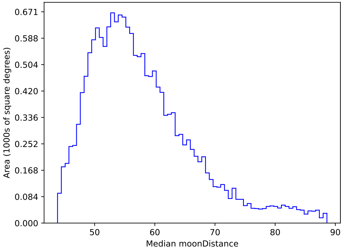
ddf_acor_sf10_lsf20_lsr20_v3.4_10yrs WFD y band: Median moonDistance
