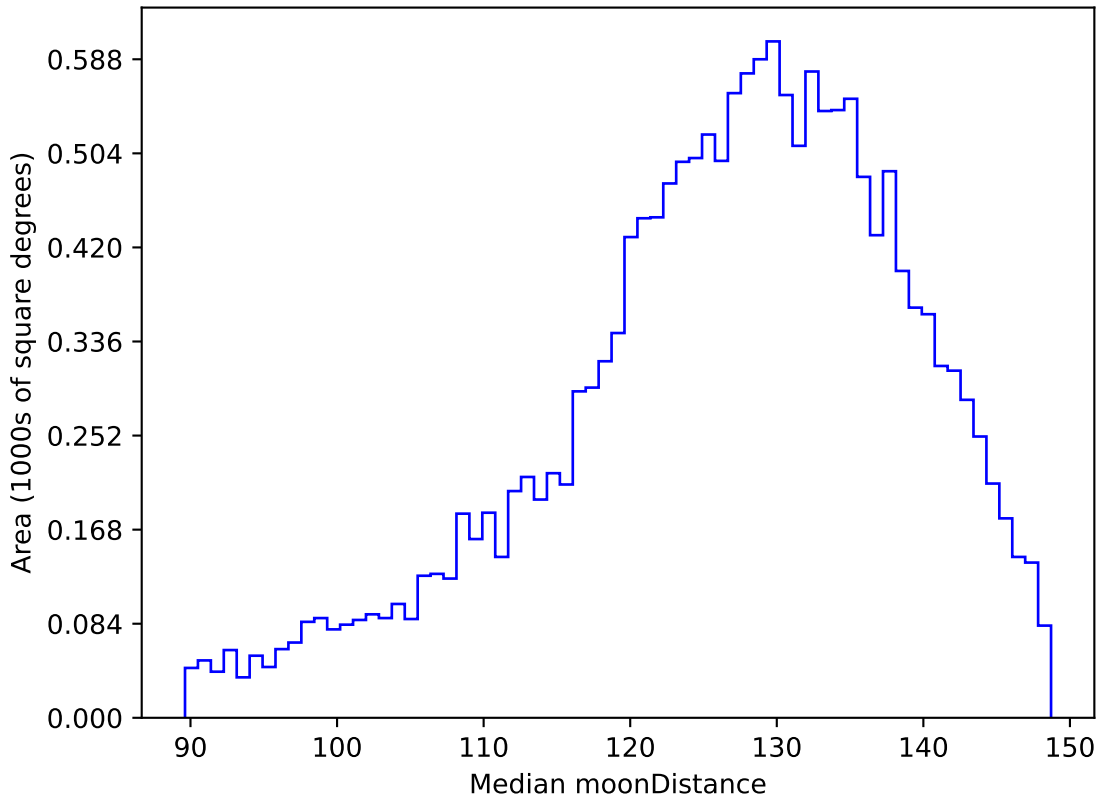
ddf_acor_sf10_lsf20_lsr20_v3.4_10yrs WFD u band: Median moonDistance
