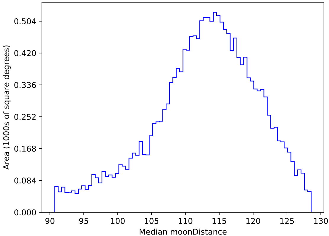
ddf_acor_sf10_lsf20_lsr20_v3.4_10yrs WFD r band: Median moonDistance
