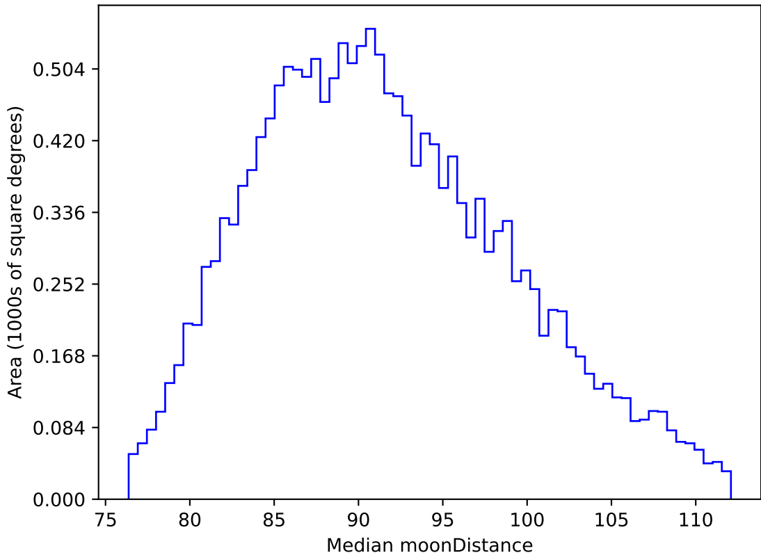
ddf_acor_sf10_lsf20_lsr20_v3.4_10yrs WFD i band: Median moonDistance
