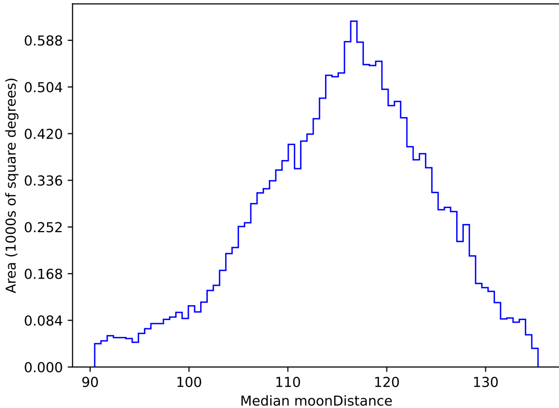
ddf_acor_sf10_lsf20_lsr20_v3.4_10yrs WFD g band: Median moonDistance
