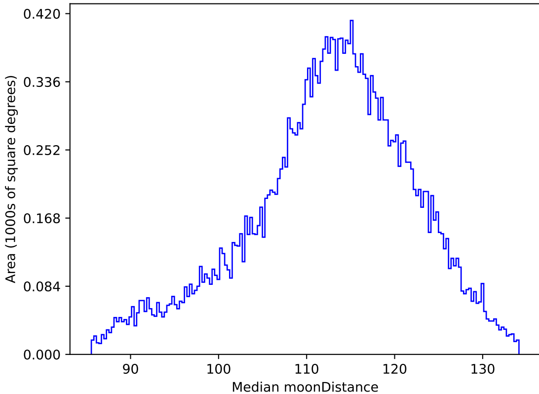
ddf_acor_sf10_lsf20_lsr20_v3.4_10yrs All sky r band: Median moonDistance
