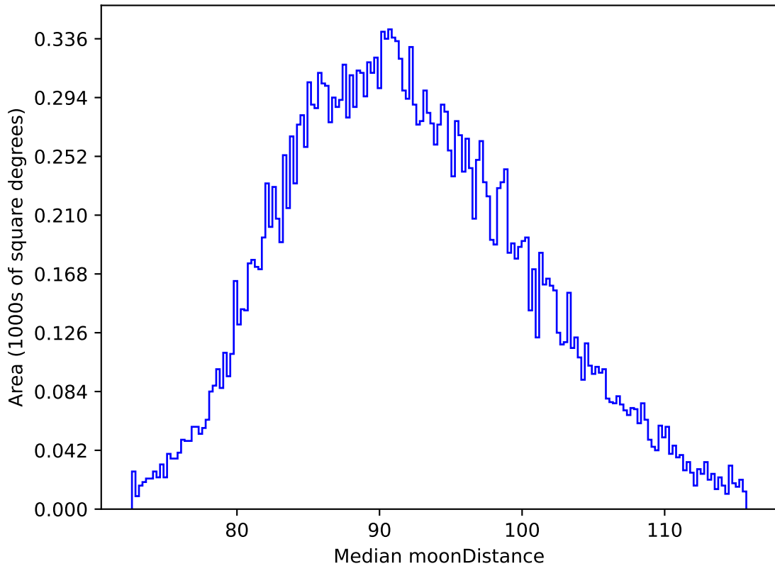
ddf_acor_sf10_lsf20_lsr20_v3.4_10yrs All sky i band: Median moonDistance
