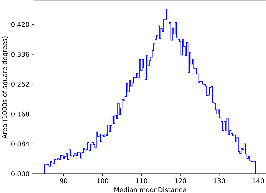
ddf_acor_sf10_lsf20_lsr20_v3.4_10yrs All sky g band: Median moonDistance
