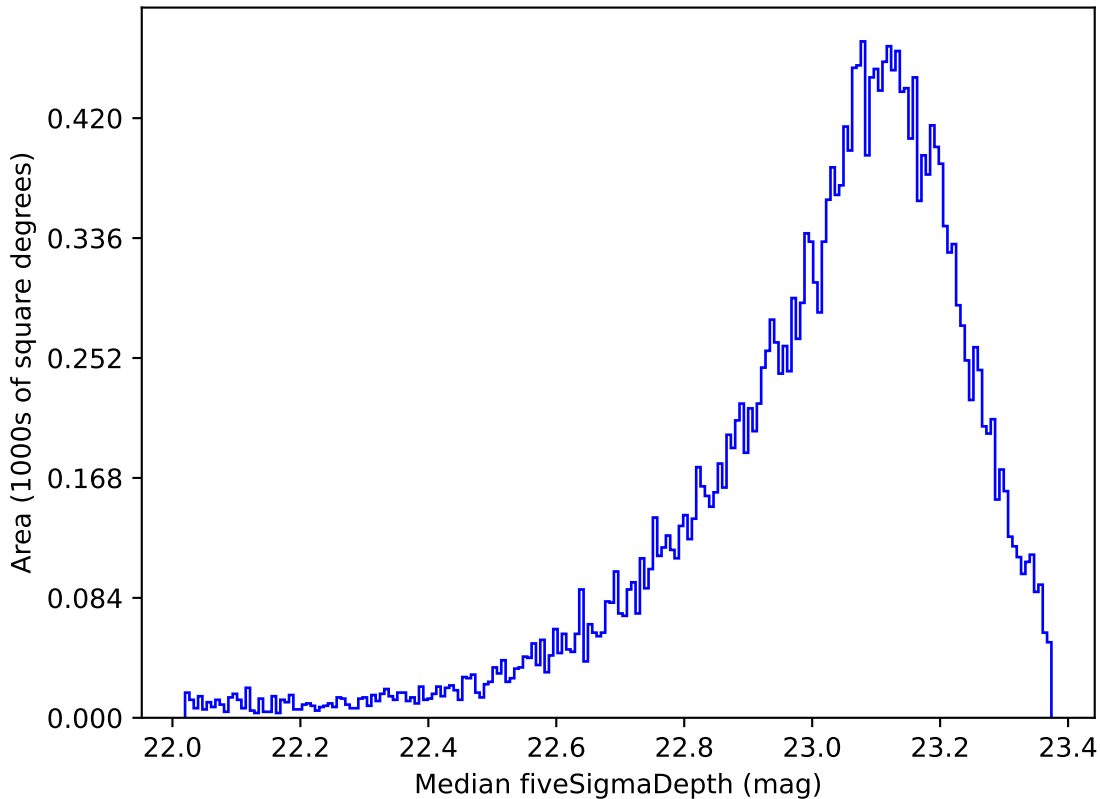
ddf_acor_sf10_lsf20_lsr20_v3.4_10yrs Yr 1 z band: Median fiveSigmaDepth
