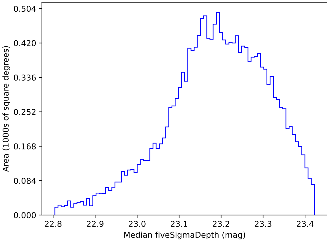
ddf_acor_sf10_lsf20_lsr20_v3.4_10yrs WFD u band: Median fiveSigmaDepth
