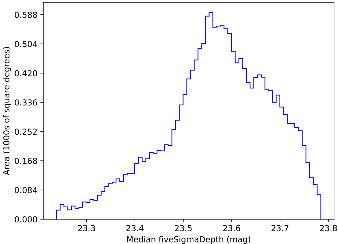
ddf_acor_sf10_lsf20_lsr20_v3.4_10yrs WFD i band: Median fiveSigmaDepth
