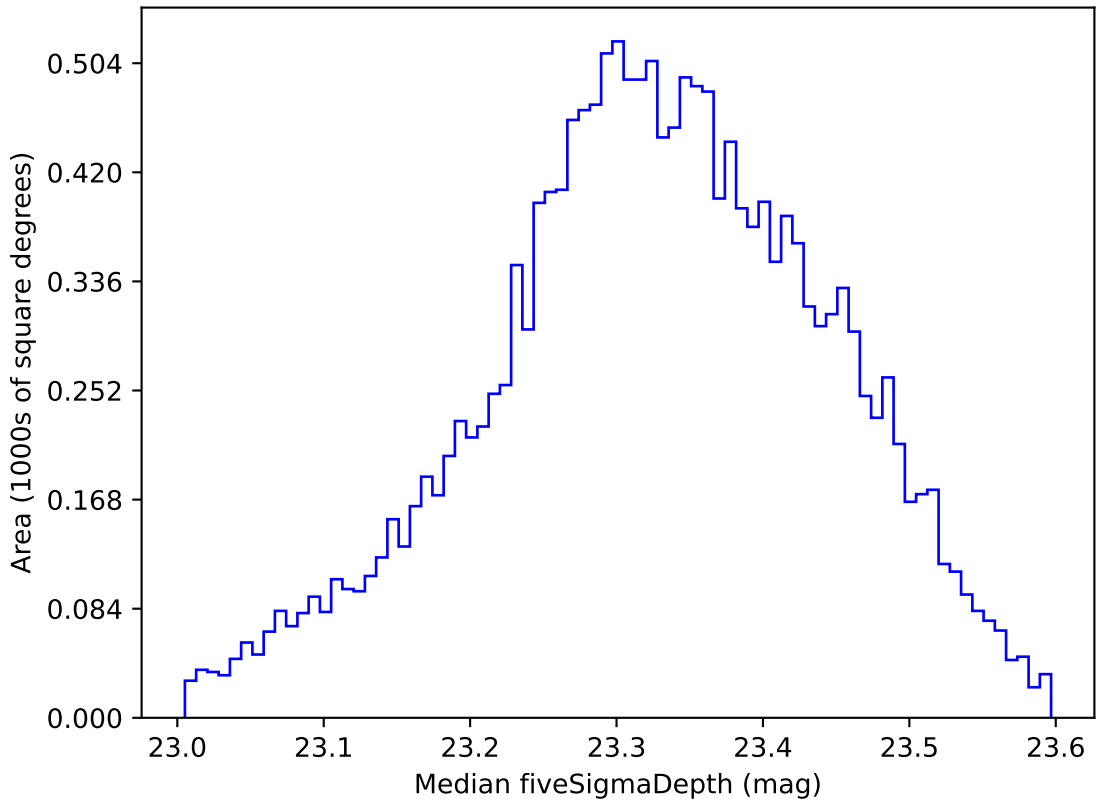
ddf_acor_sf10_lsf20_lsr20_v3.4_10yrs WFD all bands: Median fiveSigmaDepth
