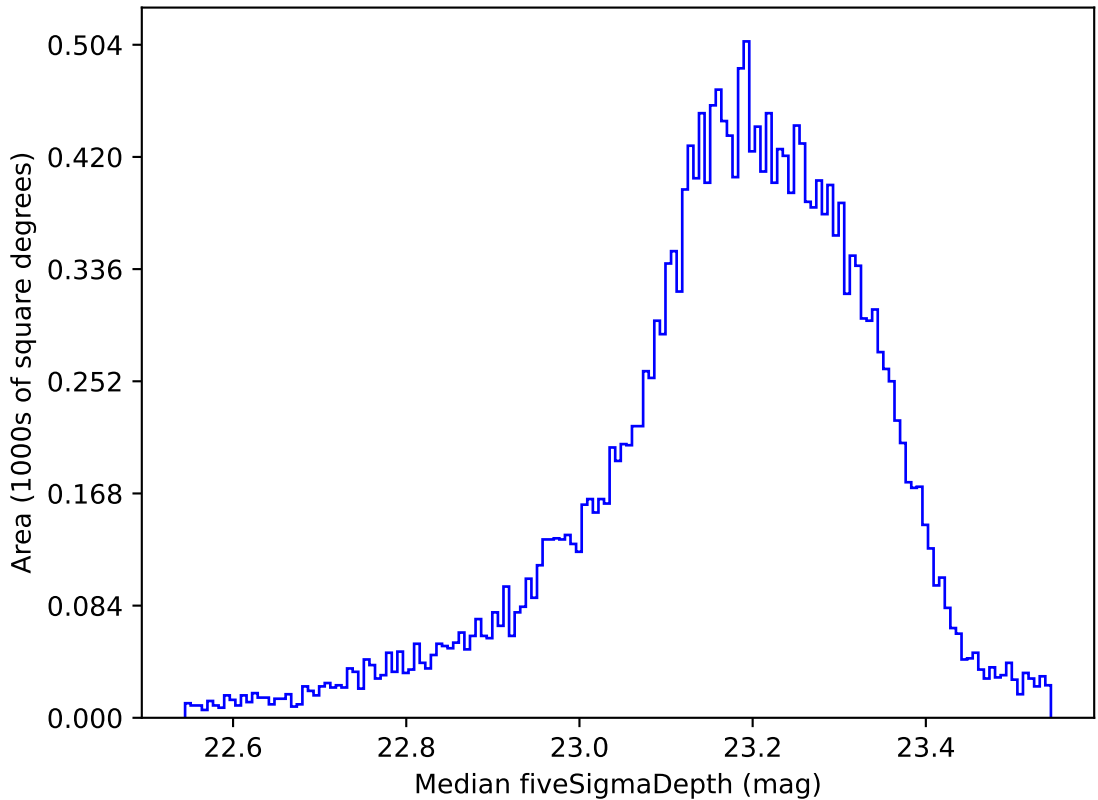
ddf_acor_sf10_lsf20_lsr20_v3.4_10yrs All sky u band: Median fiveSigmaDepth
