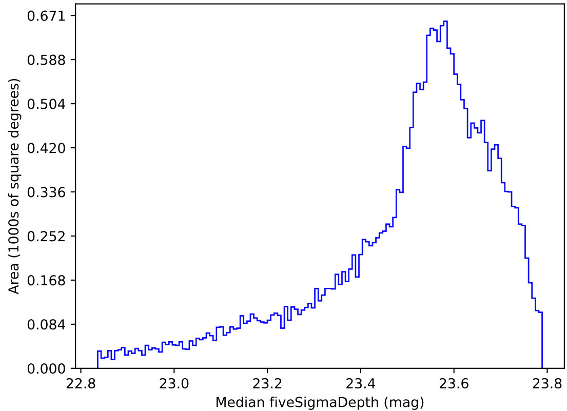
ddf_acor_sf10_lsf20_lsr20_v3.4_10yrs All sky i band: Median fiveSigmaDepth
