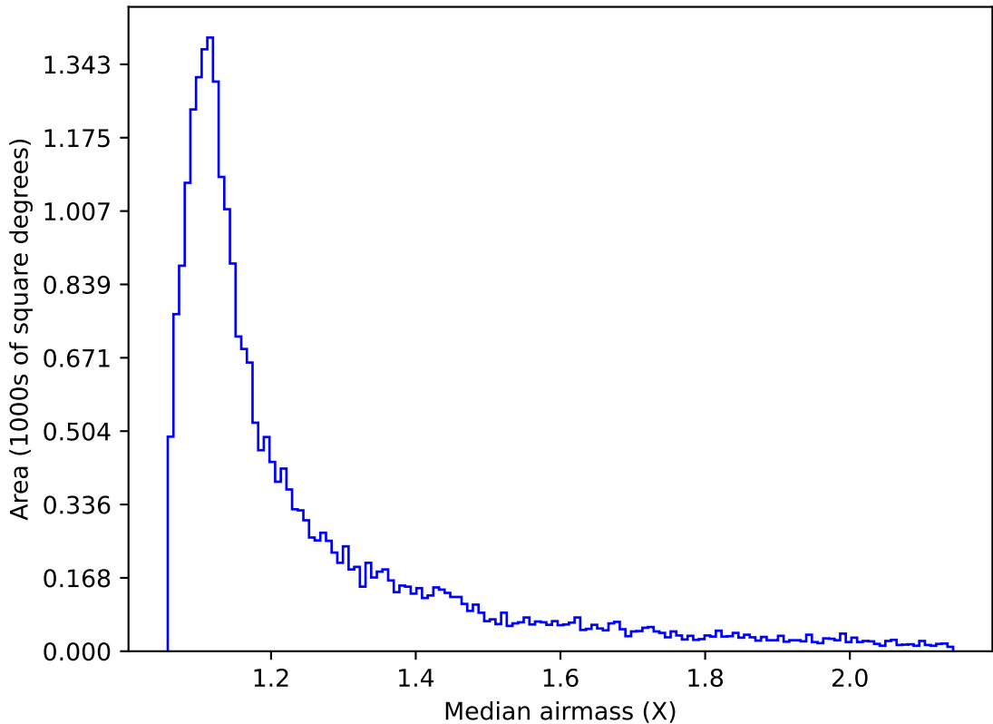
ddf_acor_sf10_lsf20_lsr20_v3.4_10yrs Yr 1 r band: Median airmass
