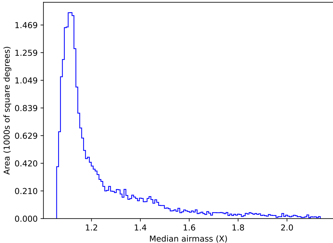
ddf_acor_sf10_lsf20_lsr20_v3.4_10yrs Yr 1 i band: Median airmass
