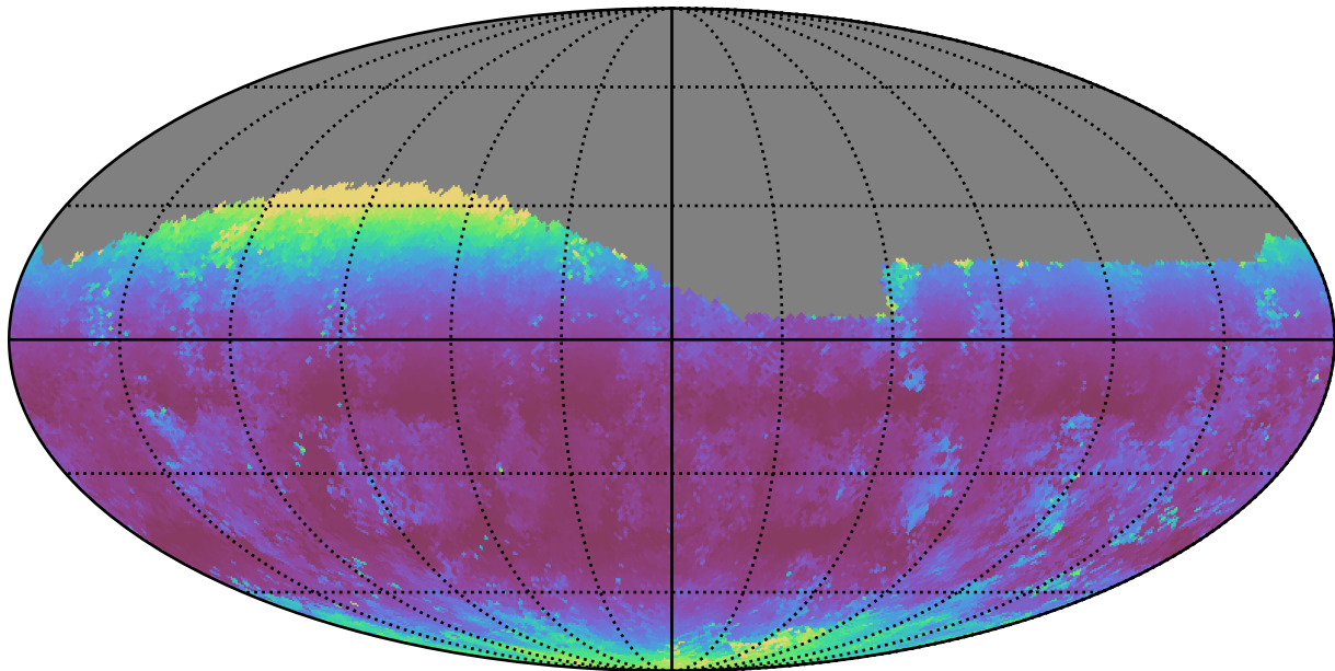
ddf_acor_sf10_lsf20_lsr20_v3.4_10yrs Yr 1 g band: Median airmass
