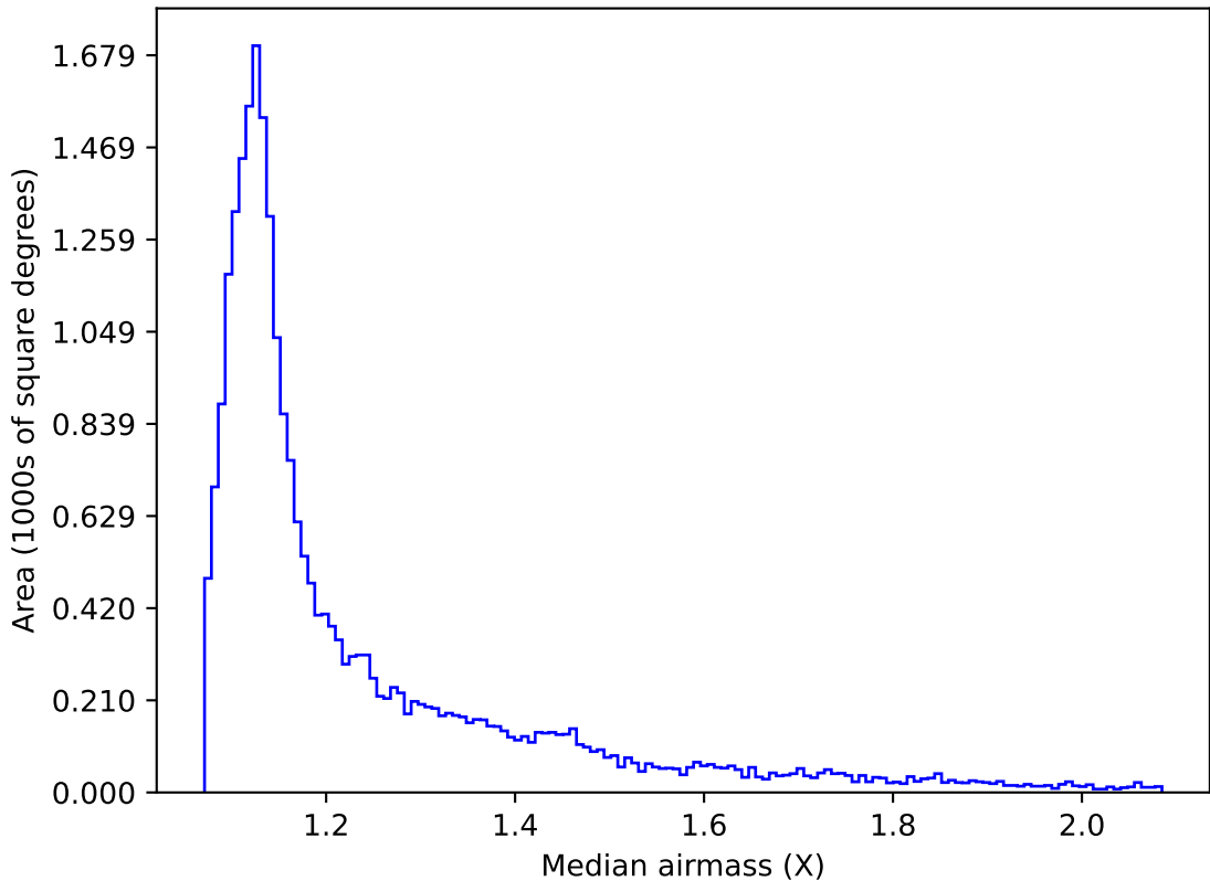
ddf_acor_sf10_lsf20_lsr20_v3.4_10yrs Yr 1 all bands: Median airmass
