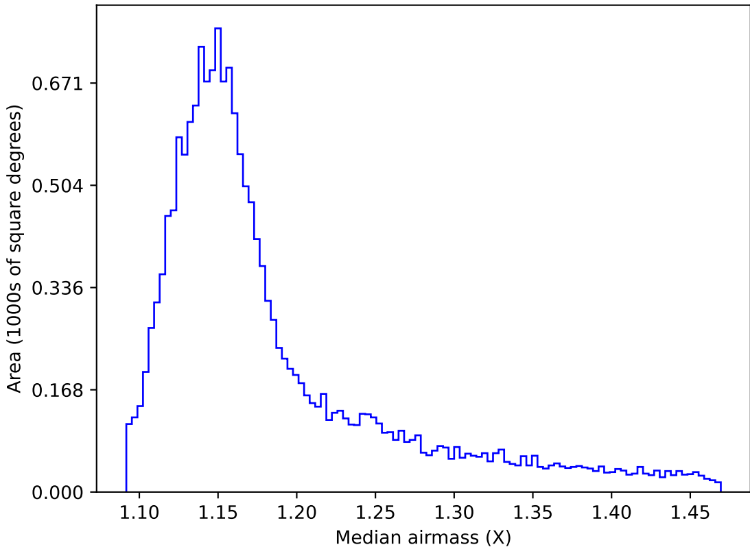
ddf_acor_sf10_lsf20_lsr20_v3.4_10yrs WFD z band: Median airmass
