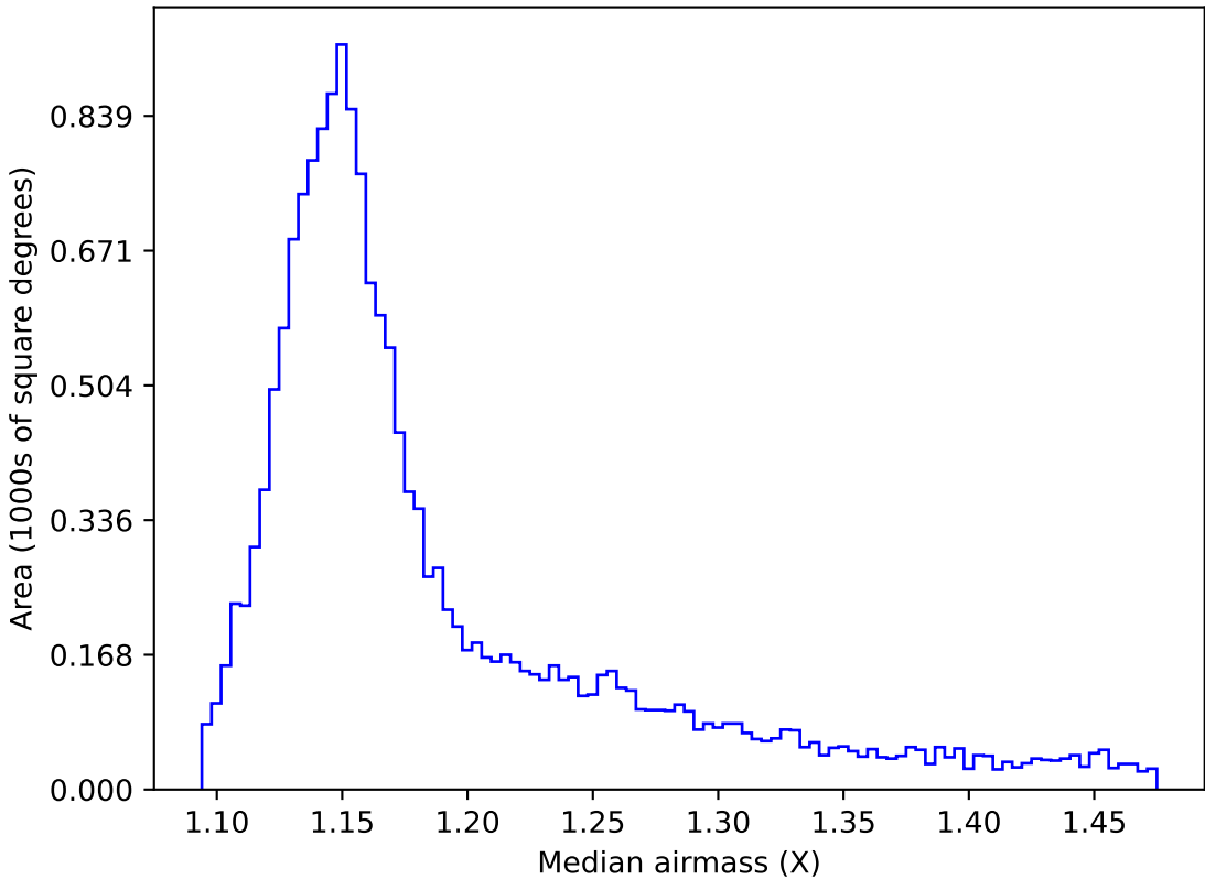
ddf_acor_sf10_lsf20_lsr20_v3.4_10yrs WFD y band: Median airmass
