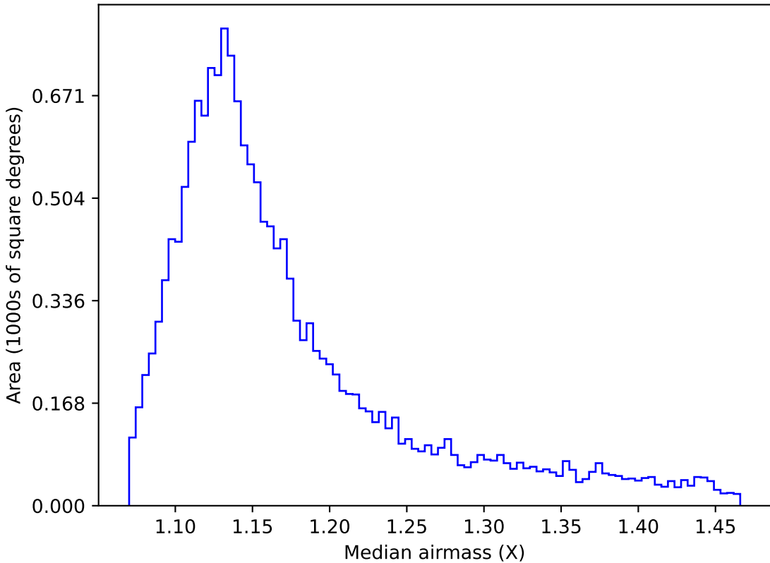
ddf_acor_sf10_lsf20_lsr20_v3.4_10yrs WFD u band: Median airmass
