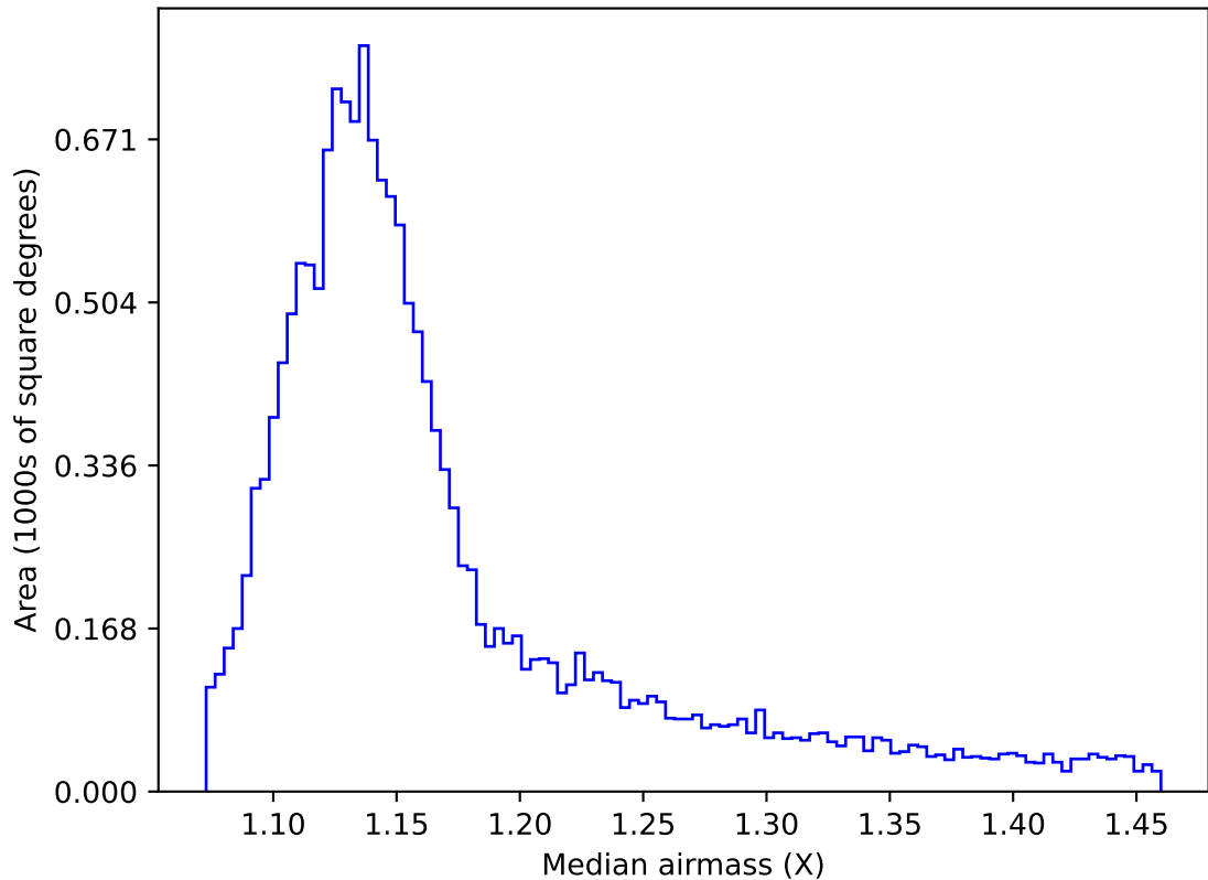
ddf_acor_sf10_lsf20_lsr20_v3.4_10yrs WFD r band: Median airmass
