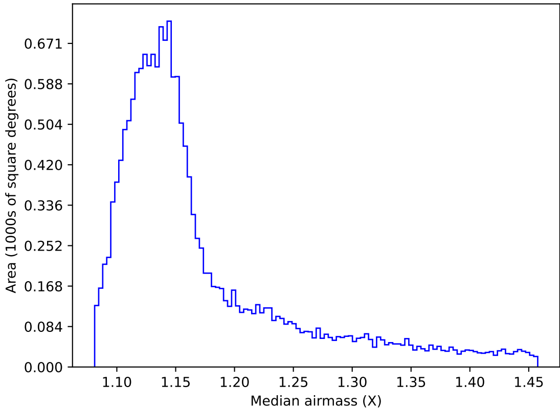
ddf_acor_sf10_lsf20_lsr20_v3.4_10yrs WFD i band: Median airmass
