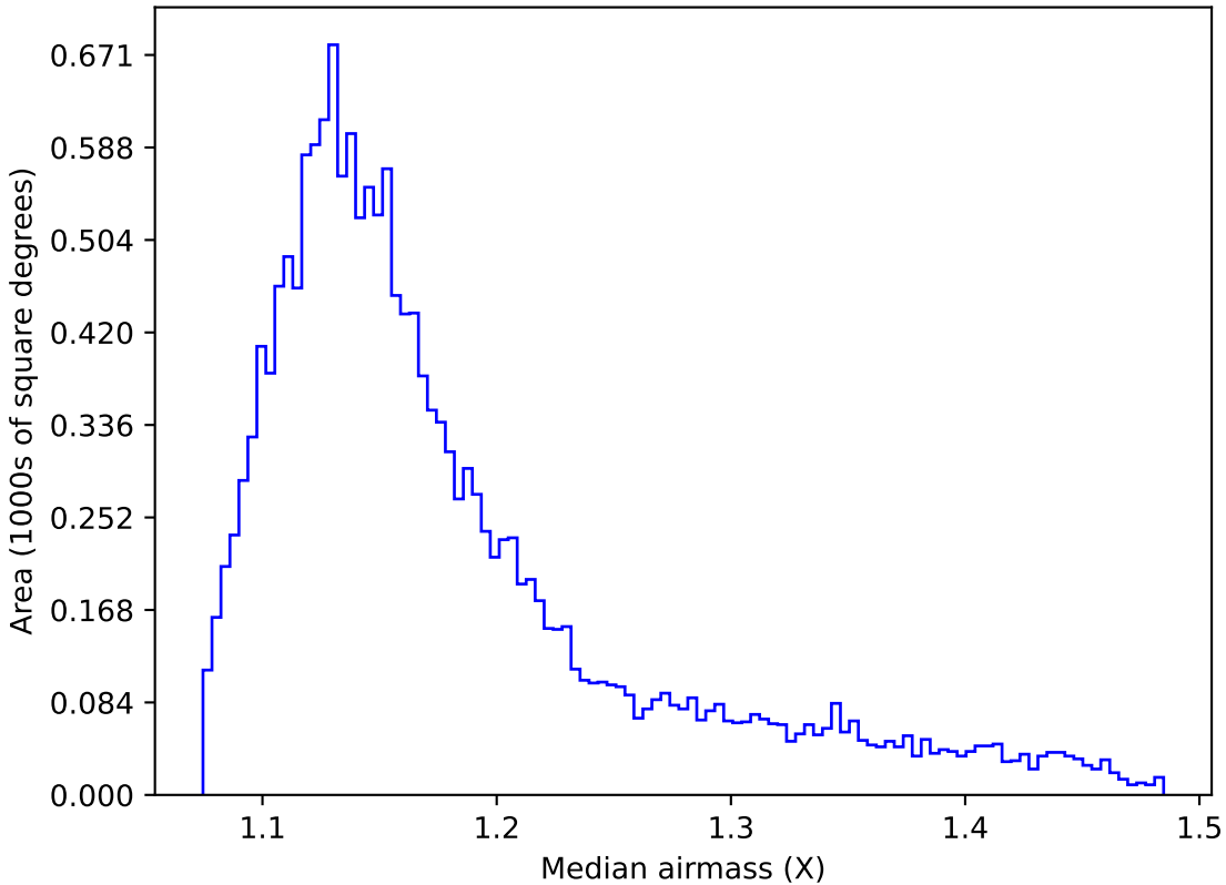
ddf_acor_sf10_lsf20_lsr20_v3.4_10yrs WFD g band: Median airmass
