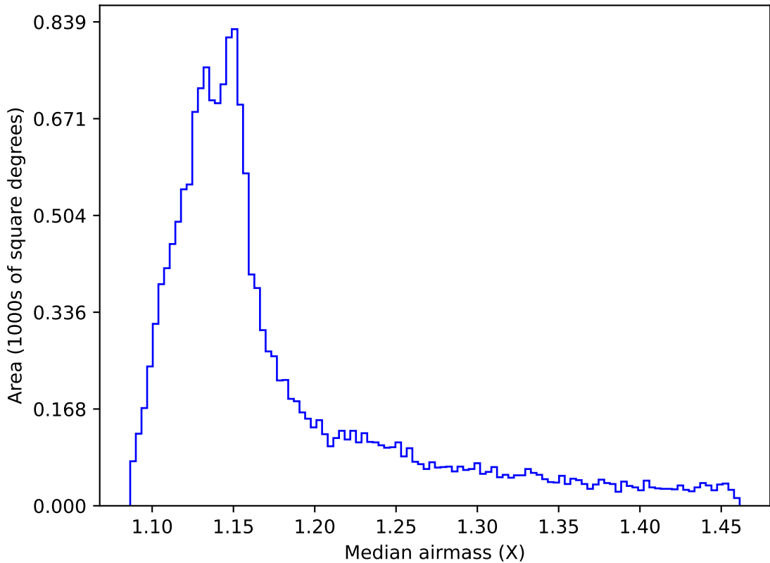
ddf_acor_sf10_lsf20_lsr20_v3.4_10yrs WFD all bands: Median airmass
