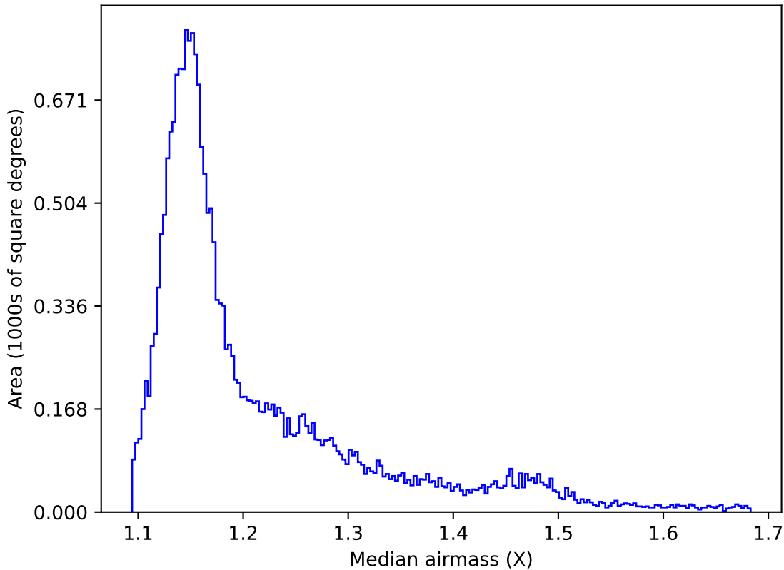
ddf_acor_sf10_lsf20_lsr20_v3.4_10yrs All sky y band: Median airmass
