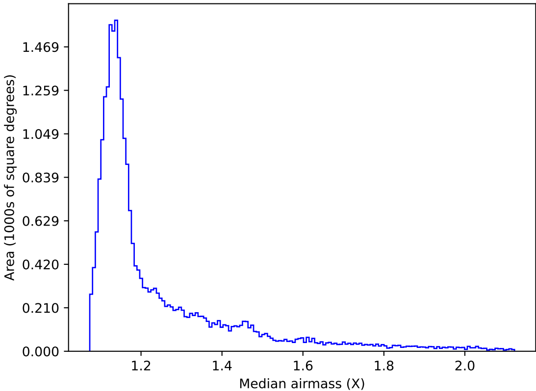
ddf_acor_sf10_lsf20_lsr20_v3.4_10yrs All sky r band: Median airmass
