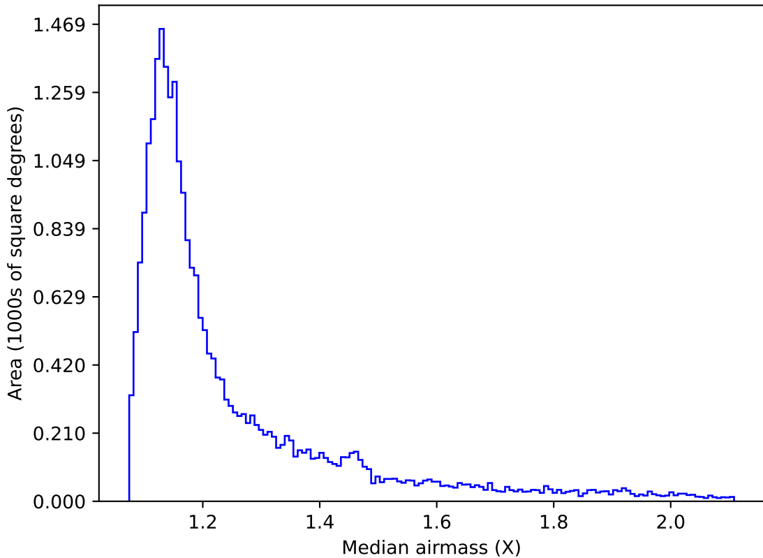
ddf_acor_sf10_lsf20_lsr20_v3.4_10yrs All sky g band: Median airmass
